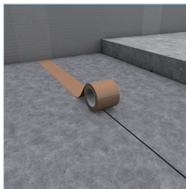
Connect joints between the wedi Nonstep ProS mats with commercially available adhesive tape.
