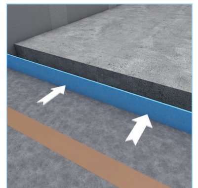
Bond wedi edge insulation strips to edges with wedi 610 then cover joints to the wedi Nonstep ProS with adhesive tape. Finished.
